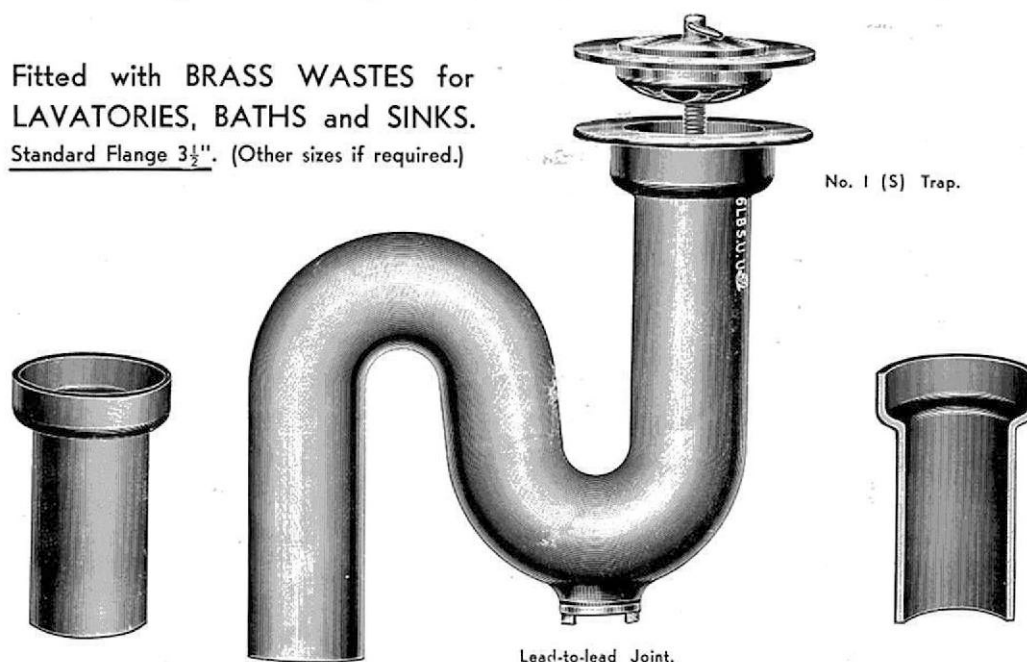
Lead-to-lead Joint.
